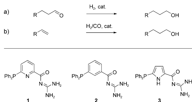
Scheme 1. a) Aldehyde hydrogenation, b) tandem hydroformylation–hydrogenation, and the structures of supramolecular ligands 1 – 3 .
